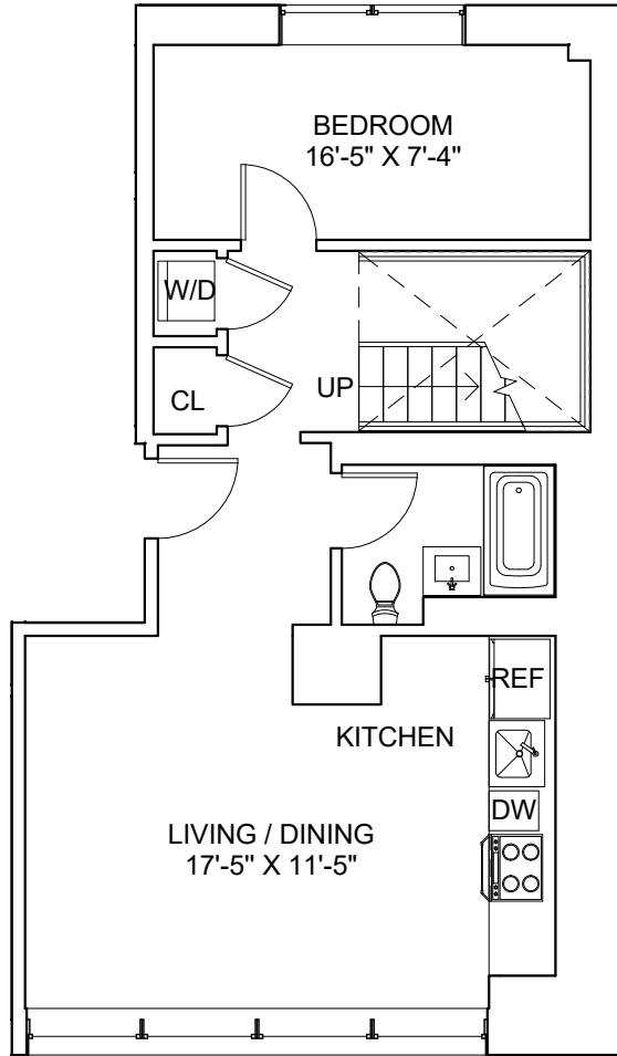
LOWER LEVEL
